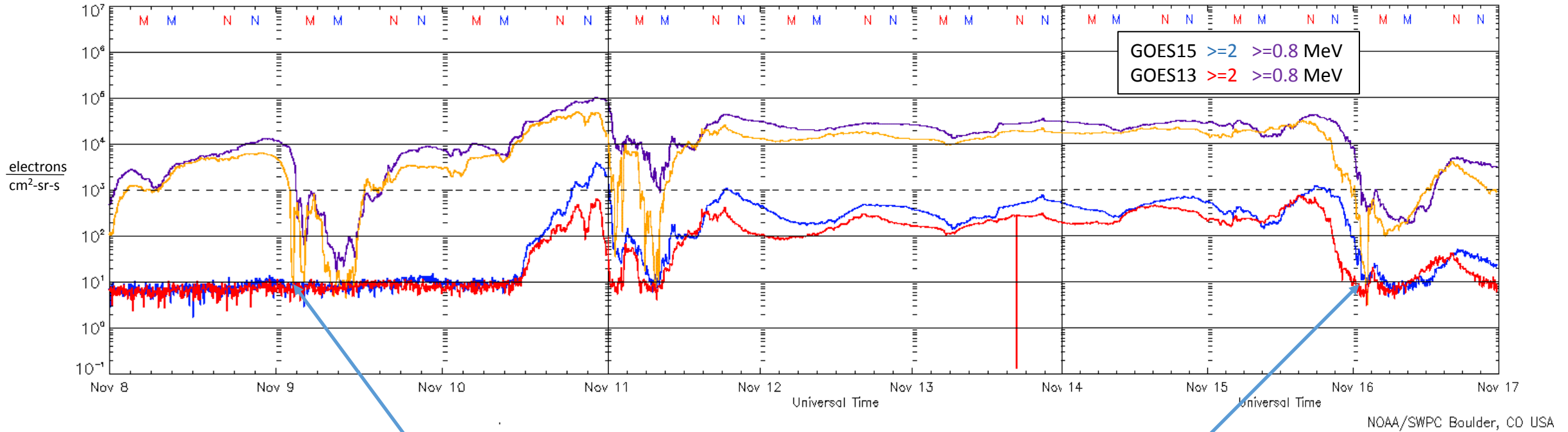
GOES Electron Flux (5 minute data)
